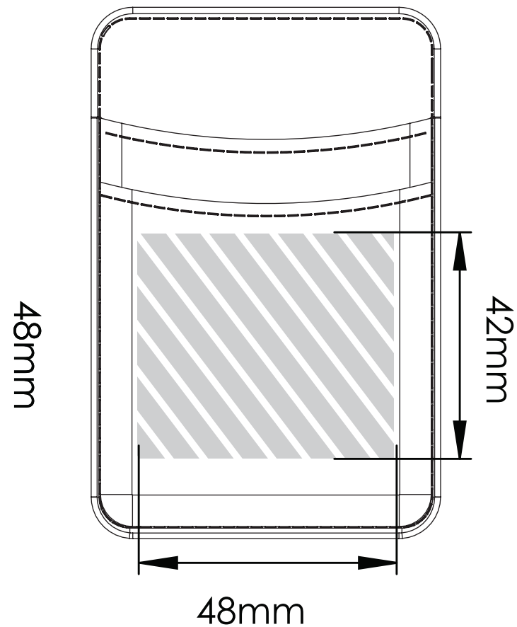
Embossing Large Setup
